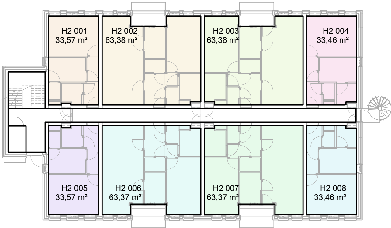
00 begane grond GO
