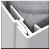
Ratchets to Lock Together
