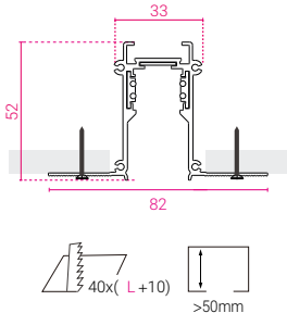
Trimless Recessed Track-EI
