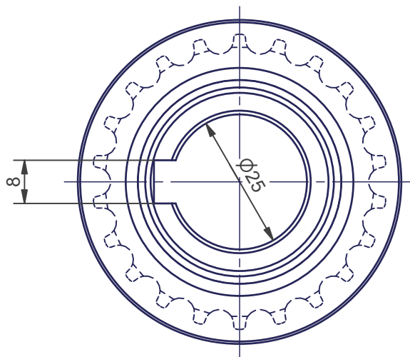
Zahnriemenscheibe 40-1803-011 (04-009-06)
